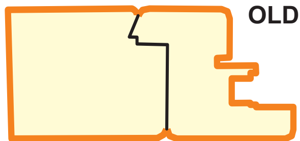
No protection at the interior of the corner joint
